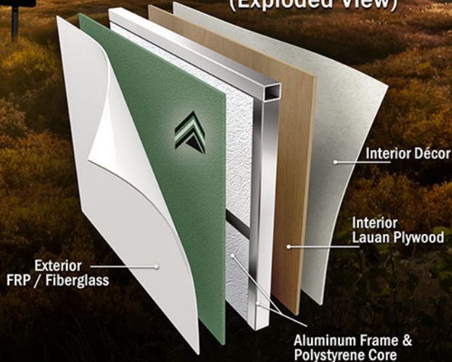
RV Sidewall Cut-Away (Exploded View)
